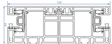
Couple rail
