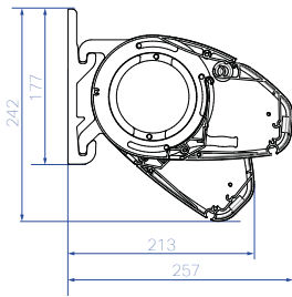
B50XL wall fixation
