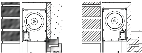
reverse mounting
