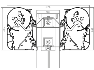
Twinstor B25
