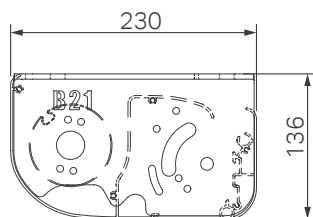
ceiling fixation B20
