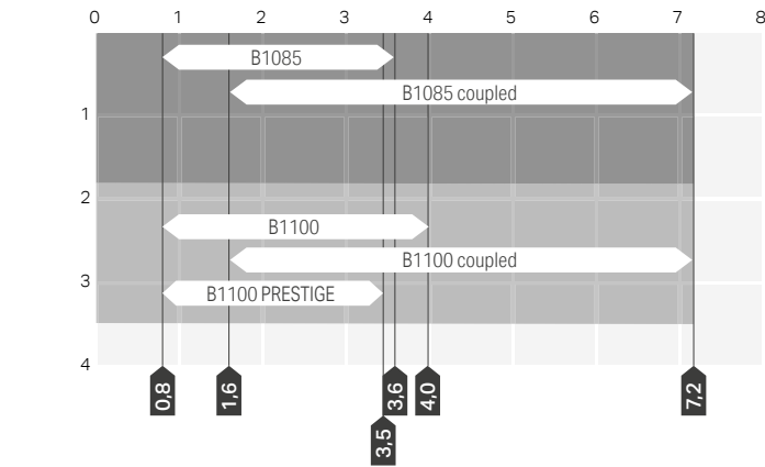
Width → Height ↓ B1085 ZIP, B1100 ZIP & B1100 ZIP Prestige Screen: max dimensions and application limits
