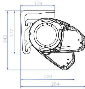
B50XL ceiling fixation
