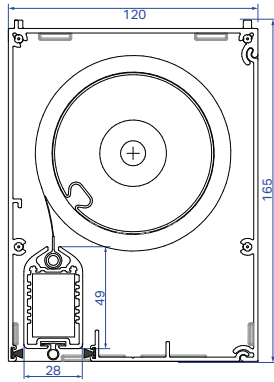
B1200 Box
