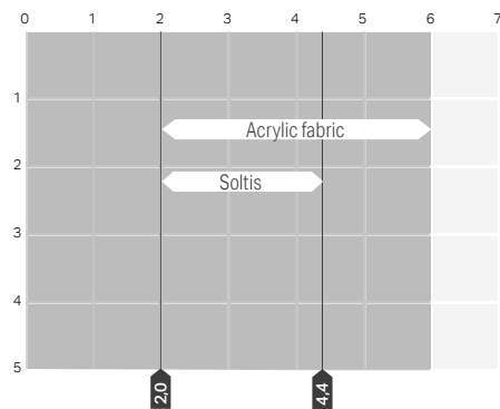
B128 Veranda: max dimensions and application limits
