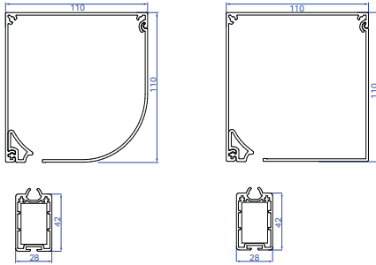
B1100 SR
