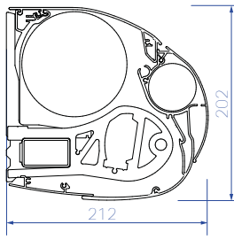
B38 Elite (Type I) Standard
