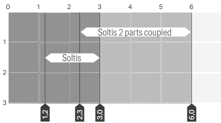
Width → Projection ↓ Topscreen: max dimensions and application limits
