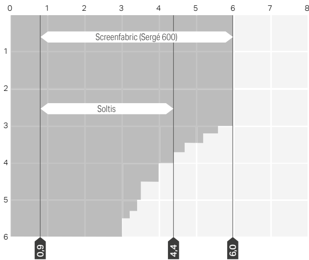
B1200 ZIP Screen: max dimensions and application limits
