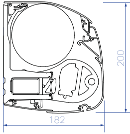
B35 Prestige (Type I) Standard
