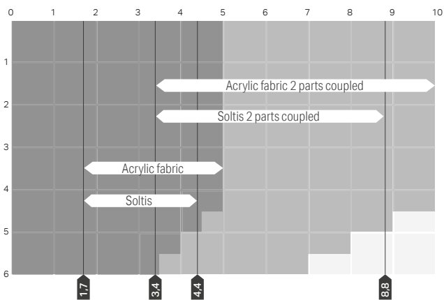
B126 Conservatory awning: max dimensions and application limits
