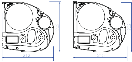
B38 Prestige (Type I) Standard
