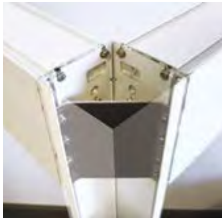
Patented corner reinforcement in the poles for rock-solid stability
