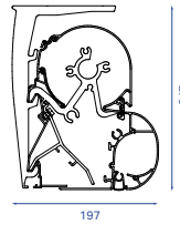
B25 ELITE / PRESTIGE VOLANT ceiling mounting
