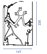
B27 ELITE / PRESTIGE wall mounting
